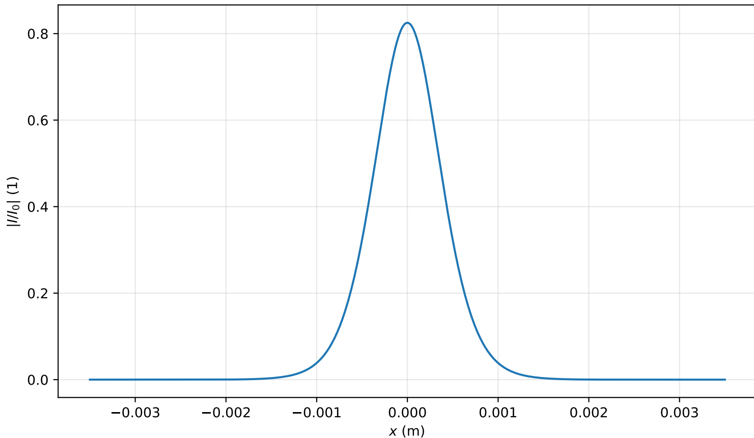
Intensity profile I(x, y = 0, z = 1.990m)/I_0 , P_{in}=0.5P_{cr} , artificial time
